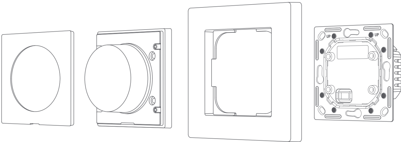
Switch Plate
